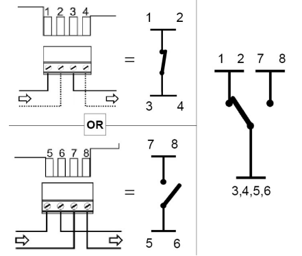
CONNECTION DETAILS
